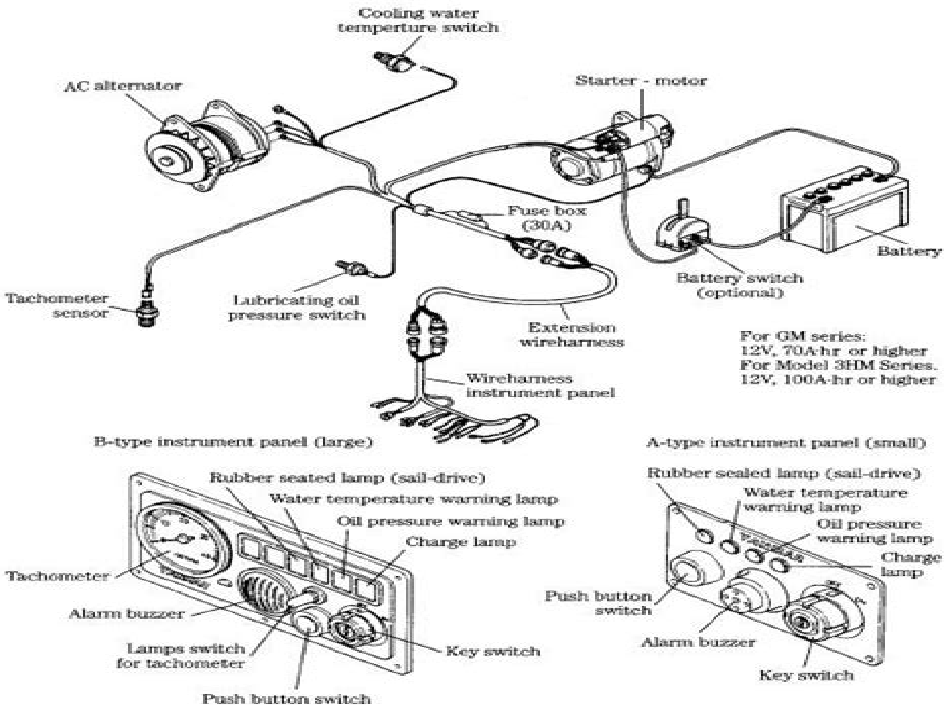
11-3 Wiring layout for a Yanmar Marine application.
