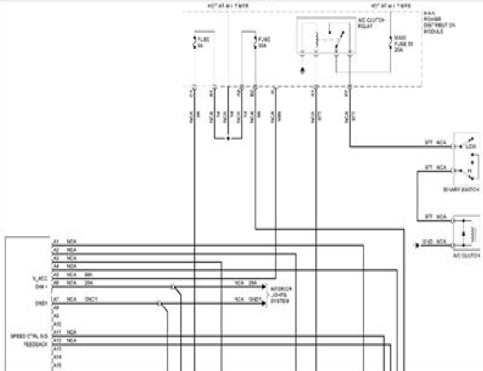
Fig. 1: AC Circuit (1 of 2)
