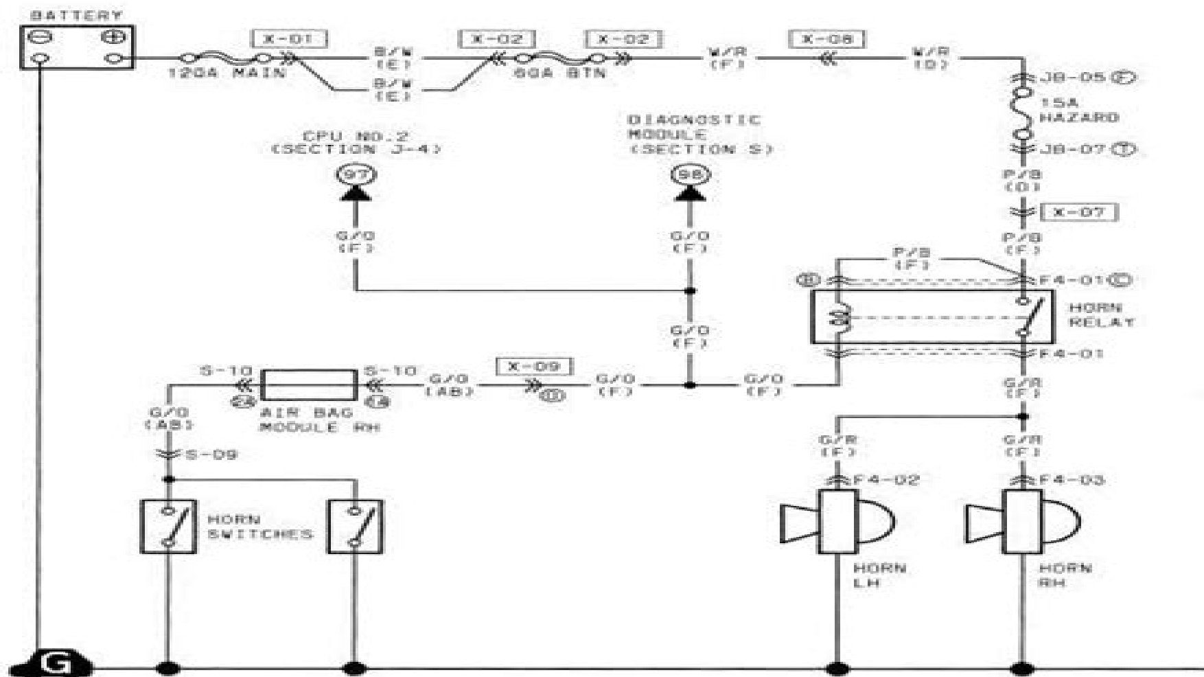
F4-01 HORN RELAY (F)
