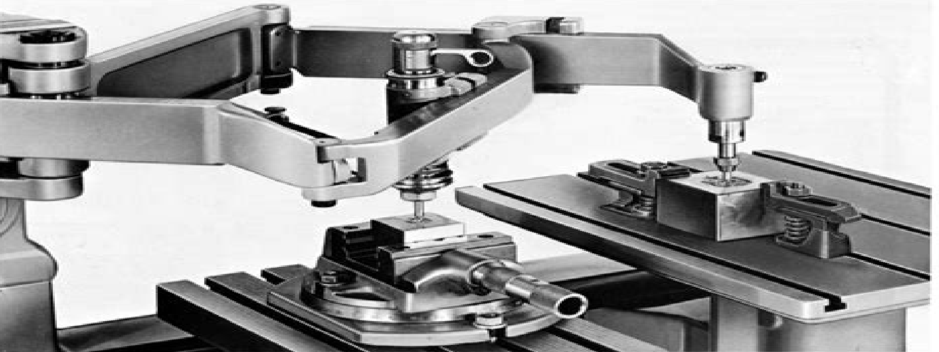
Fig 6 Reducing an escutcheon die from a steel master (GK 12)
