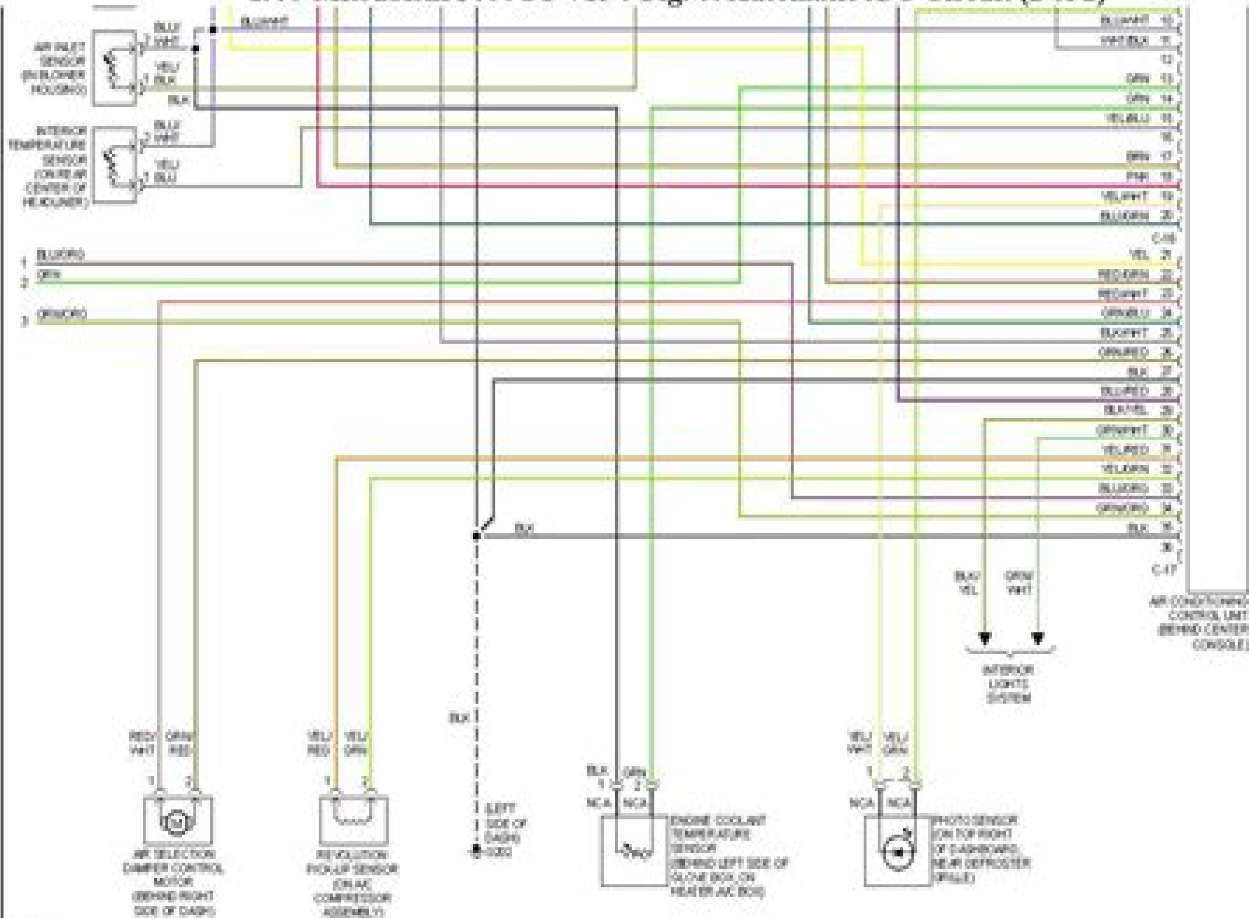
1999 Mitsubishi 3000GT VR-4-Fig. 6: Automatic A/C Circuit (2 of 2)
