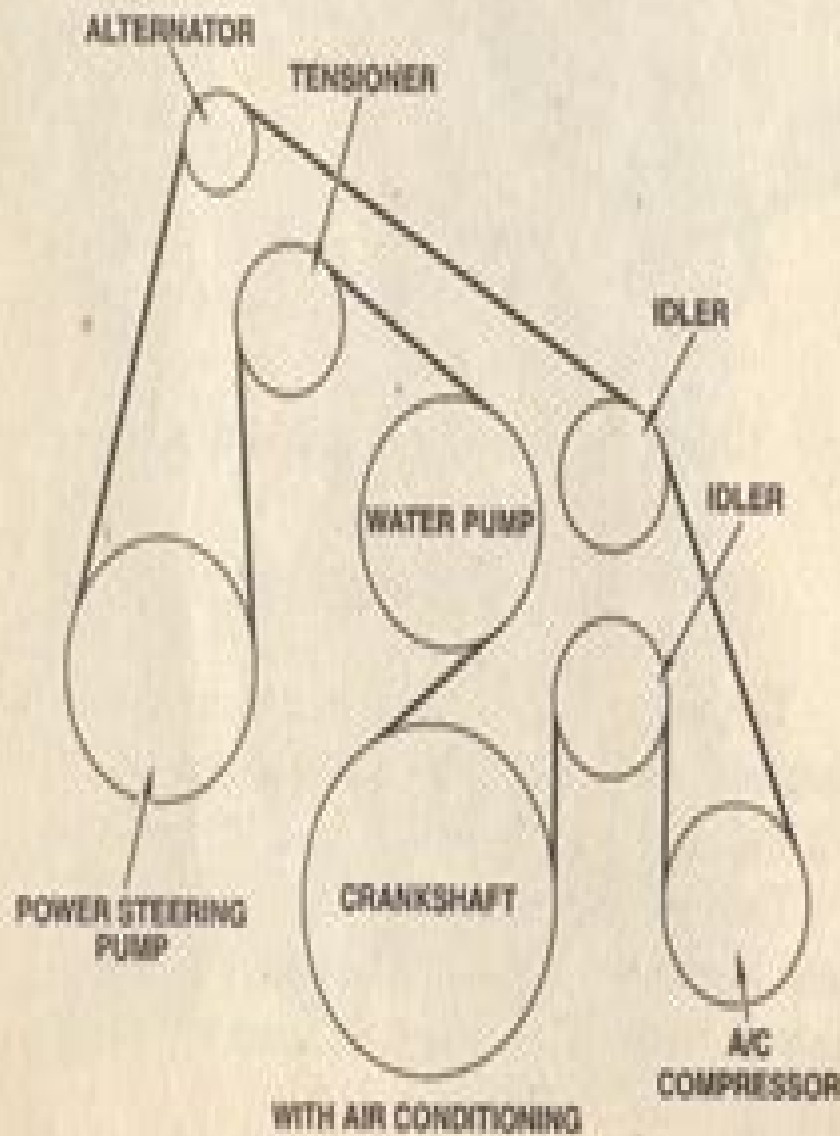
Drive belt installation schematic.
