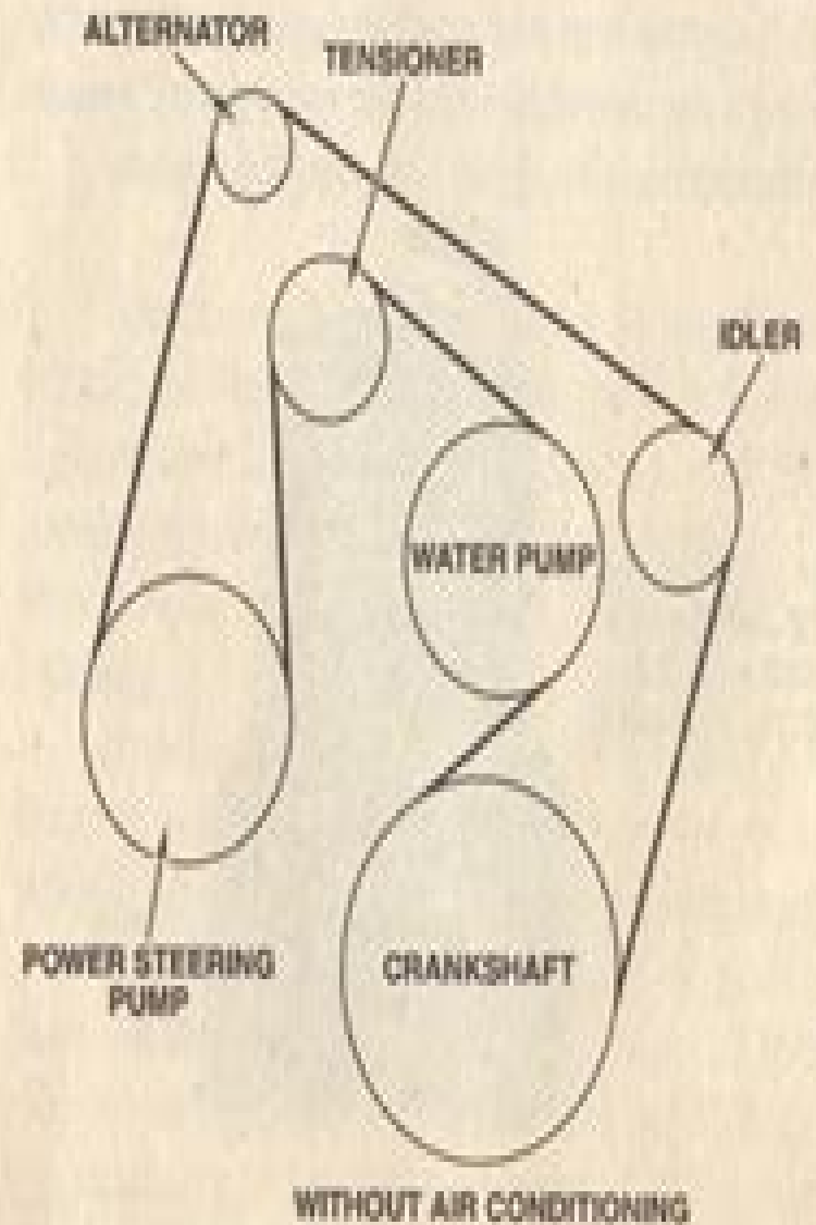
Drive belt installation schematic.
