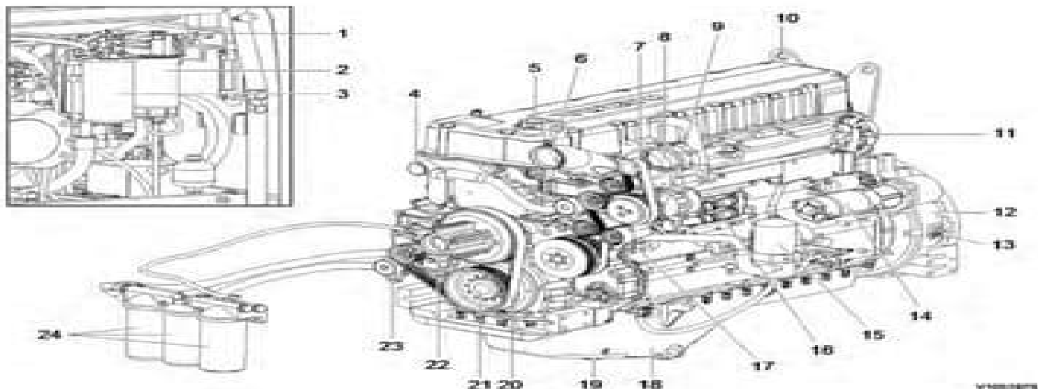
Figure 1 Engine, structure
