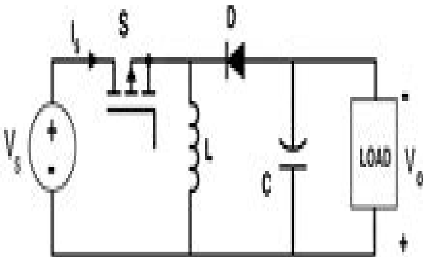
Buck-Boost Converter
