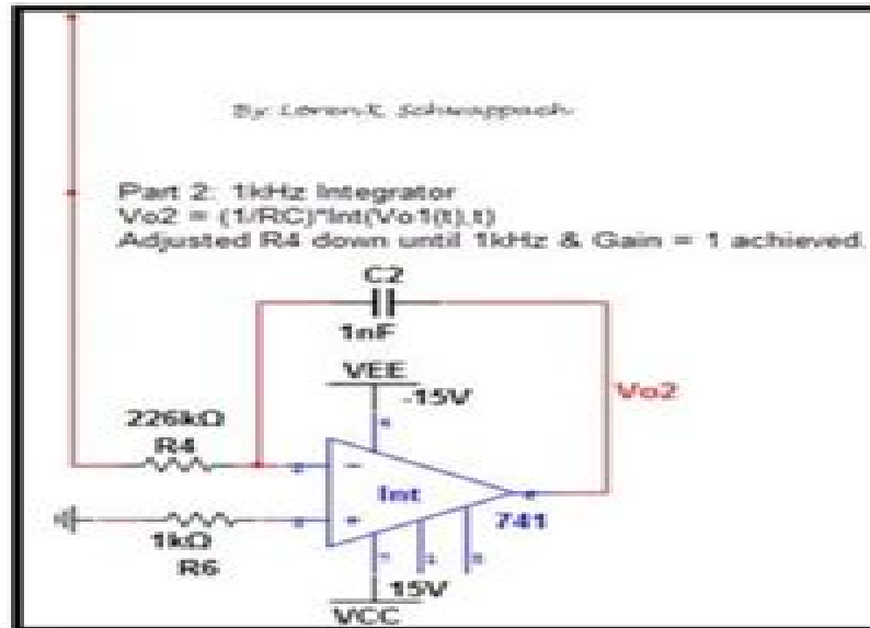
Figure 4: Multisim 1 KHz Integrator, designed the same as the integrator in lab #1 but using different RC values.
