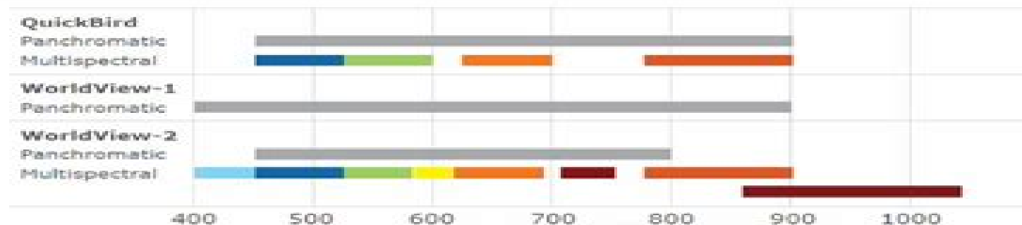
Fig.1. Spectral Bands of DigitalGlobe's Satellites
