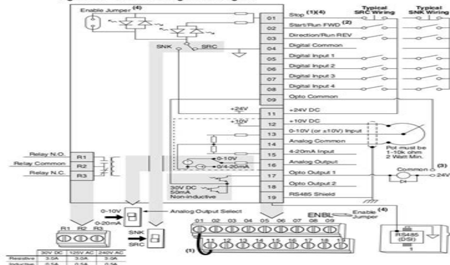
Figure 1.5 Control Wiring Block Diagram
