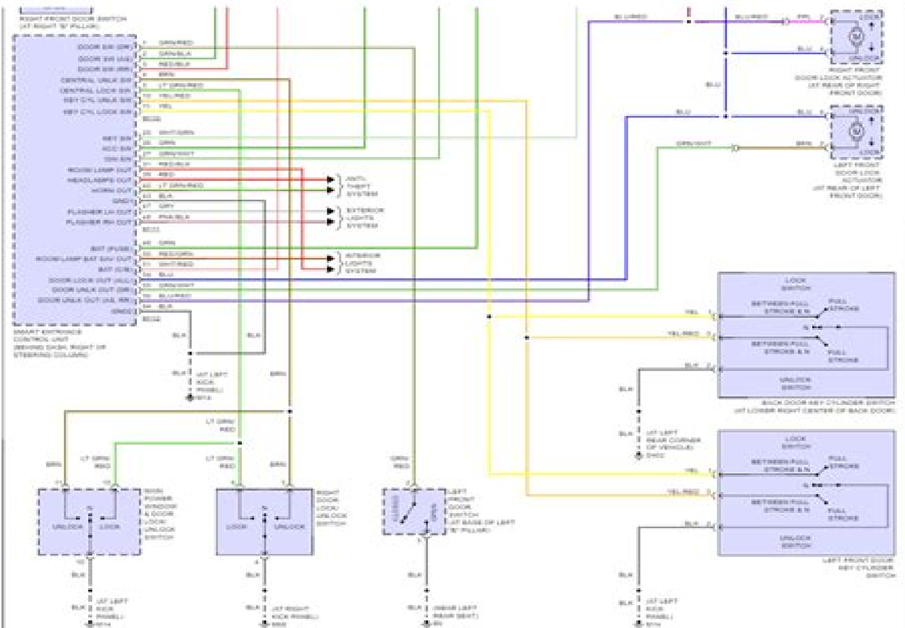
Fig 1: Power Door Locks Circuit
