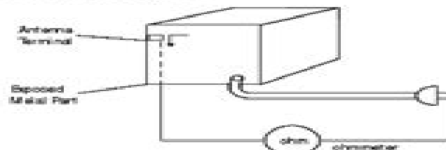
Fig. 1-2 Insulation Resistance Test
