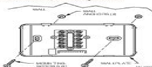
Fig. 2. Mounting wallplate to wall.
