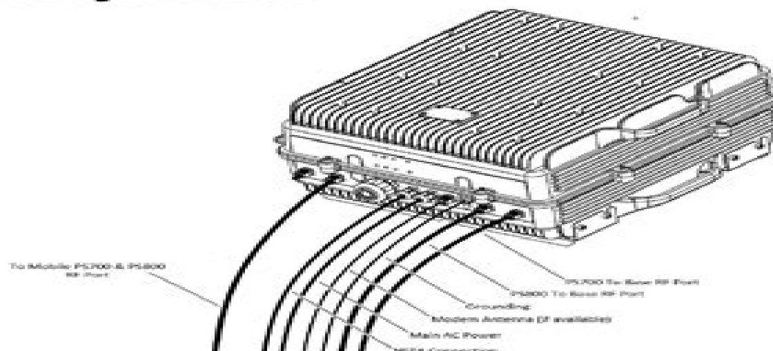
Figure: RF ports and Power Cable Glands location
