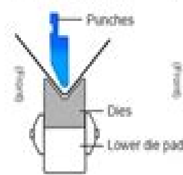
90° Kneebend (Thick plate) Plate thick: 4~10mm
