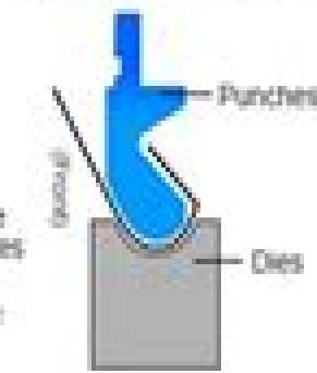
R Kneebend (2 processes) Plate thick: 1.2~1.5mm
