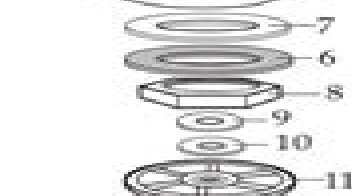
503171 Container with Blending Assy. (current production)
