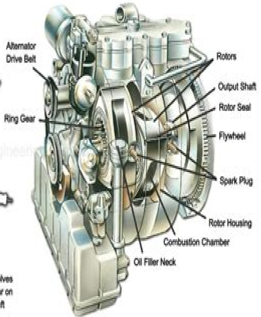
Wankel Engine (Rotary Wankel Engine)
