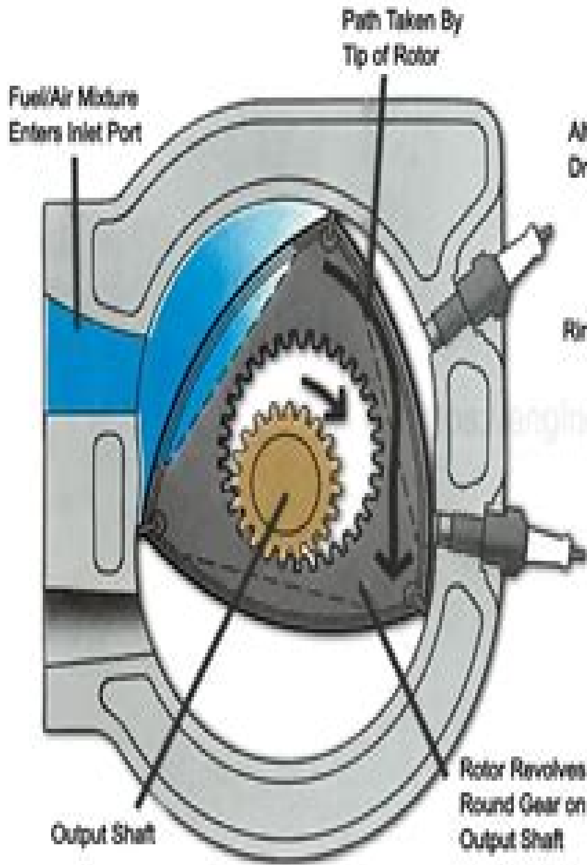
Wankel Engine (Rotary Wankel Engine)
