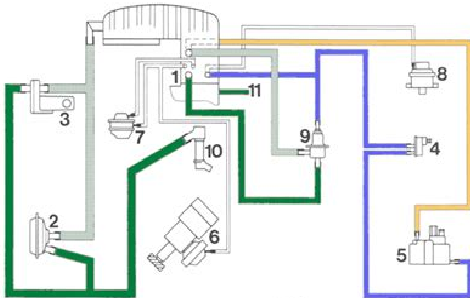
Vacuum line and emission control component layout of 1978 models
