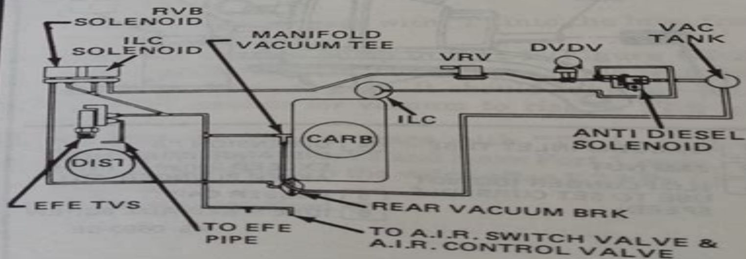
Figure C2-20 - ILC/RVB Vacuum System
