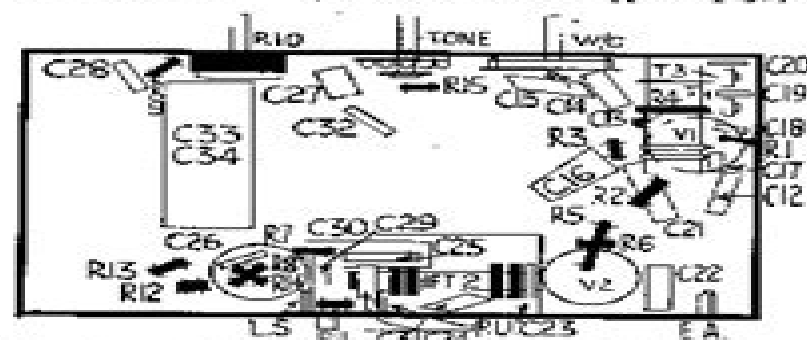
Layout diagram of the MP chassis (condensers on right) identifying components. Condensers are in outline and resistors in solid black to aid reference.
