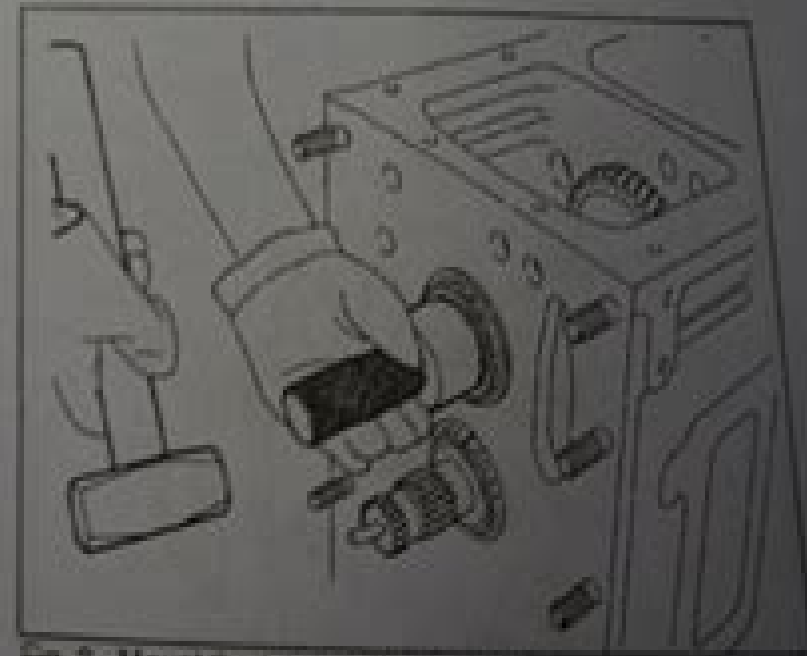
Fig. 8 - Mount the taper roller bearing;
