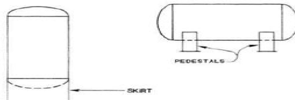
Figure 12-3. Vessel support devices.
