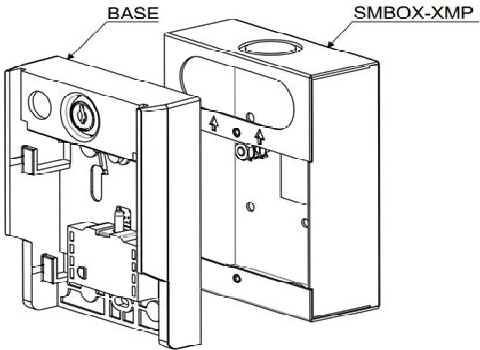
Figure 1 Mounting the X-Series pull stations onto the SMBOX-XMP
