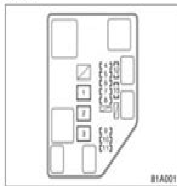
Engine compartment
