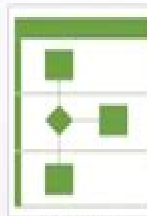
Cross-Functional Flowchart
