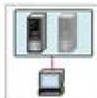
Enterprise Application
