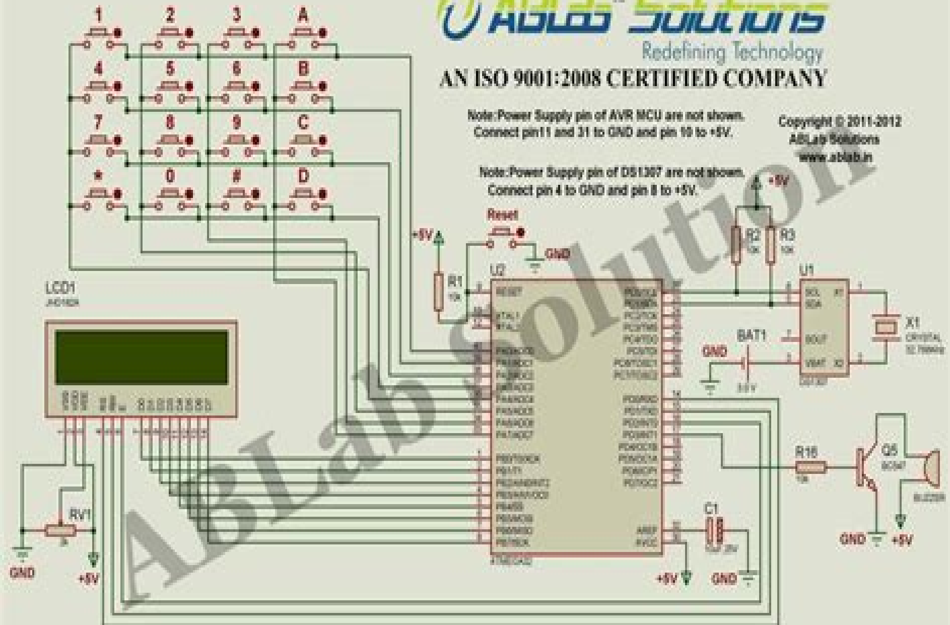
Circuit Diagram of DS1307 RTC based Alarm Clock Designing with ATmega32 and LCD Display
