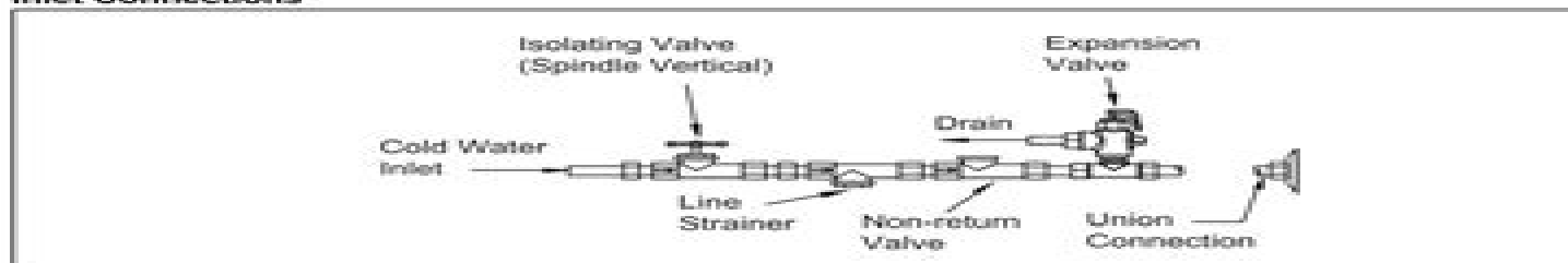
Figure 2 - Inlet Connections
