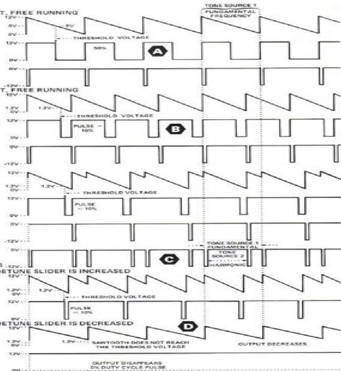
FIGURE 1 TYPICAL TONE SOURCE WAVEFORMS
