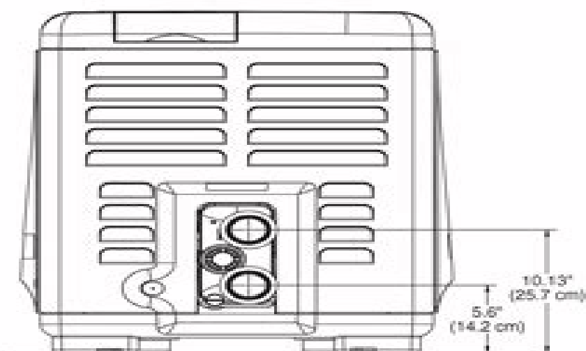
PLUMBING SIDE
