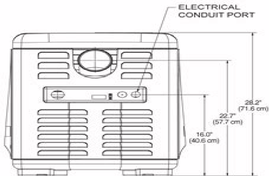
EXHAUST SIDE
