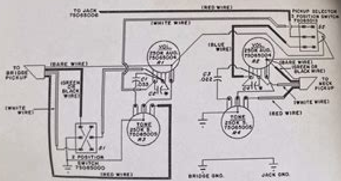
T-40 & T-60 ® WIRING DIAGRAM REAR VIEW
