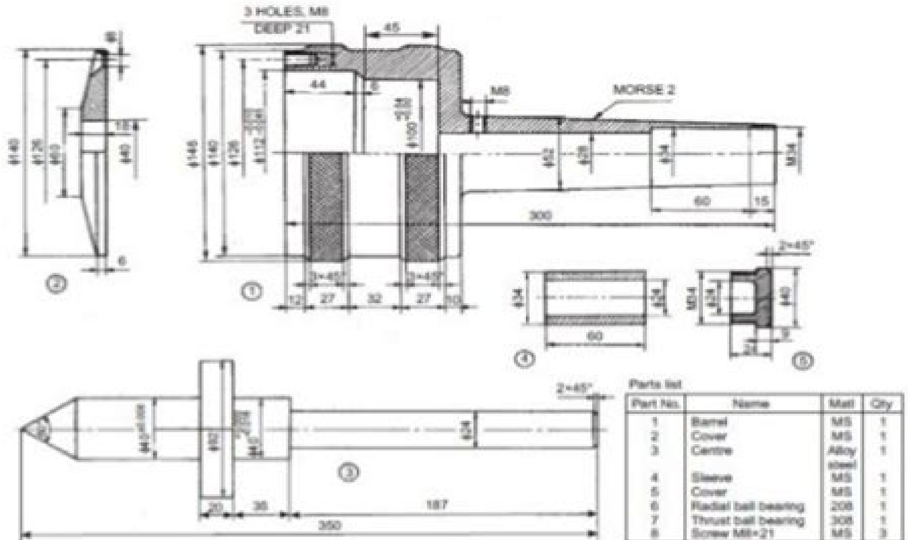
Fig. 18.26 Revolving centre
