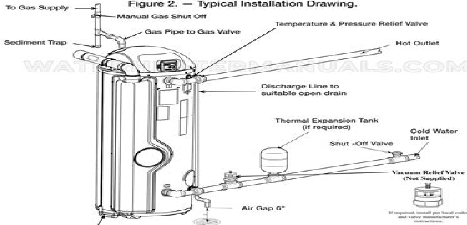
Figure 2. — Typical Installation Drawing.
