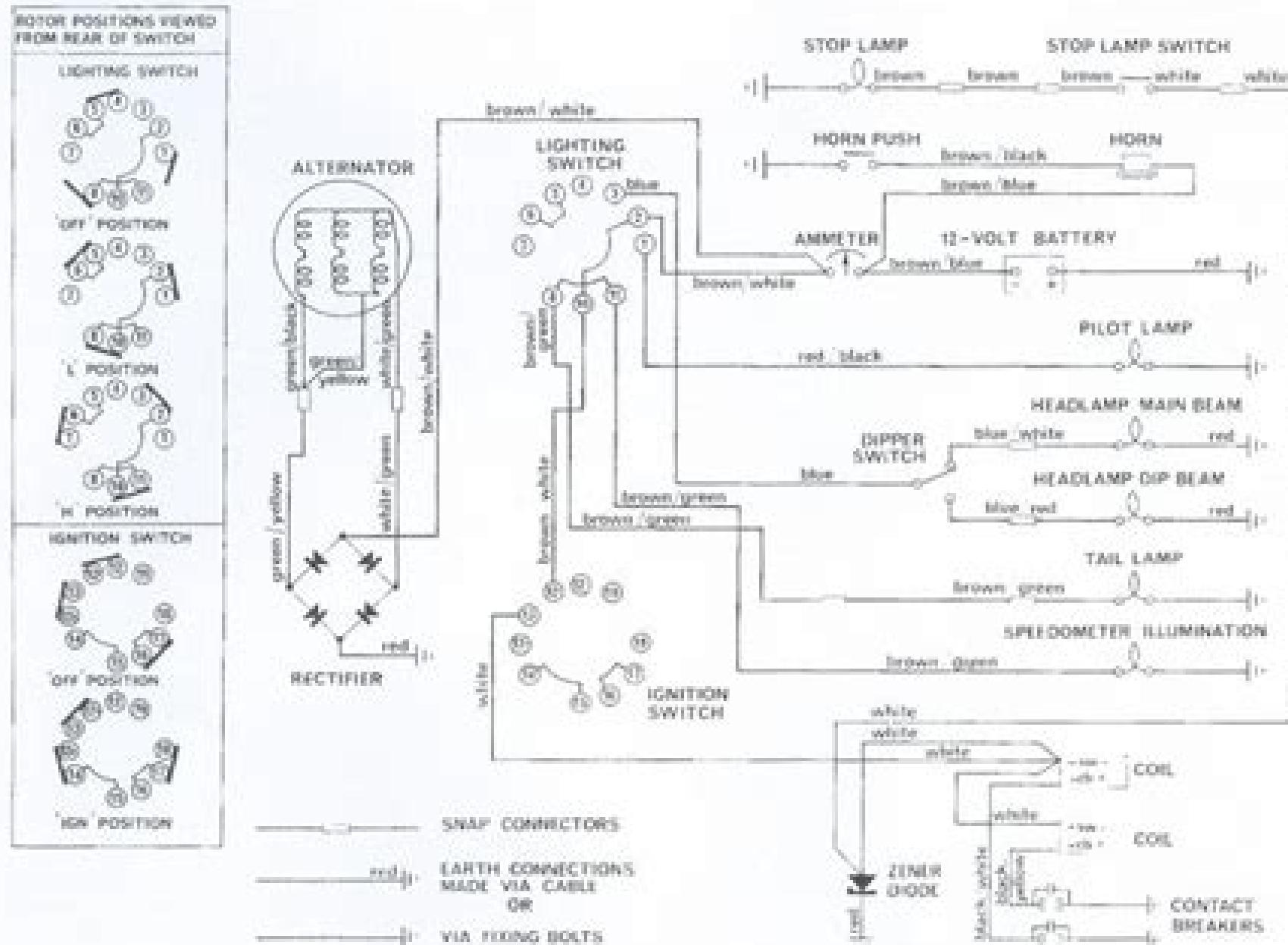
Fig. H34. Wiring diagram—Coil ignition 12 volt models with nacelle from engine number DU2M75
