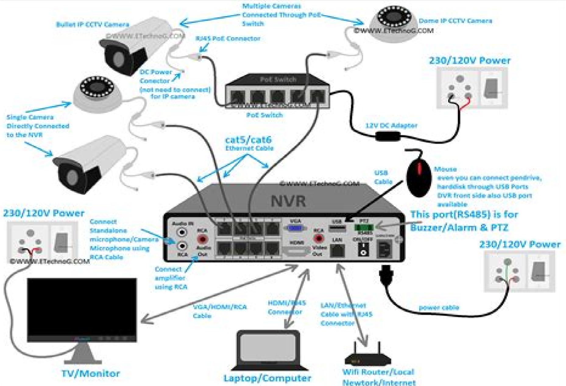
Figure. 01 IP CCTV Camera Wiring Diagram for Installation with NVR
