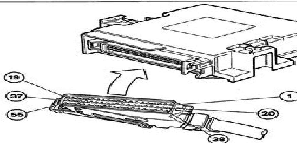
Identifying connections on control unit (pin-out)
