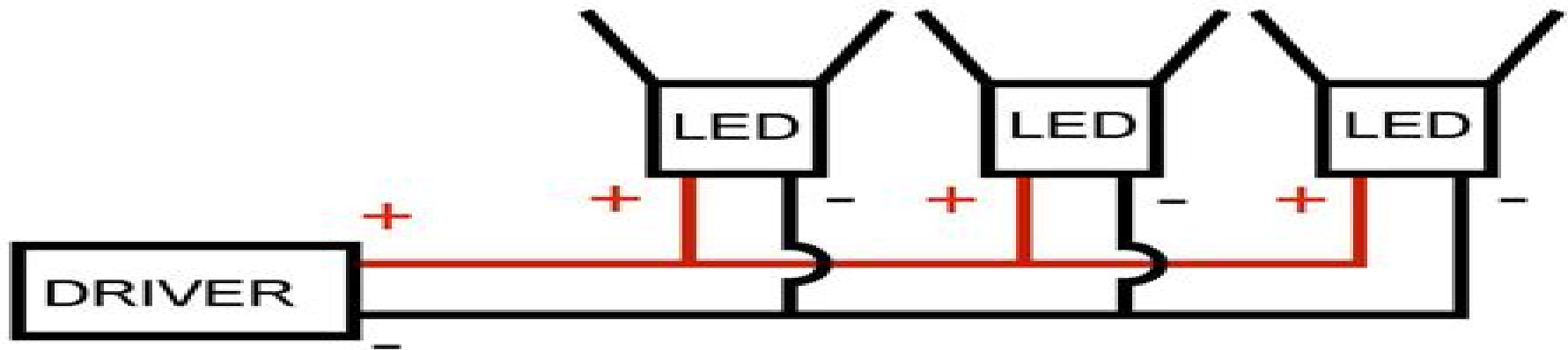
PARALLEL WIRING CONSTANT VOLTAGE
