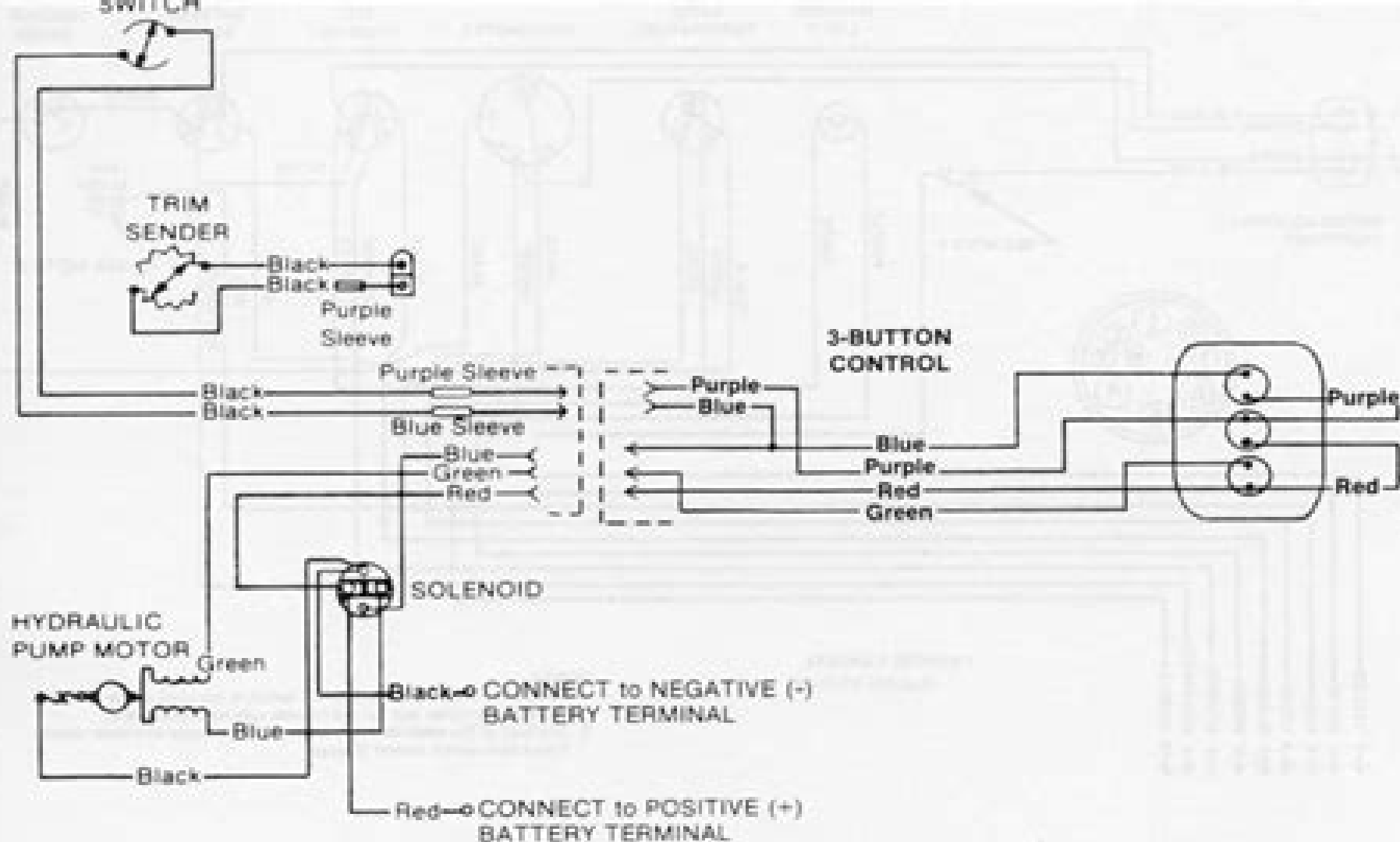
MerCruiser Wiring Diagram - Power Trim Circuit (Single Solenoid System)
