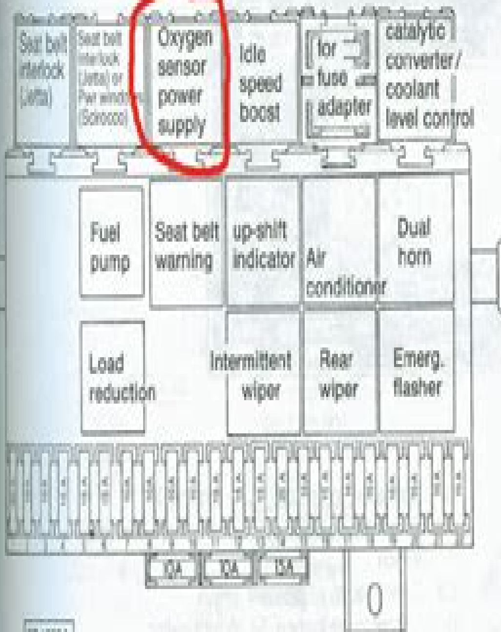
Fig. 12-4. Relay locations on 1982 Scroccos (above). Relay locations on 1983 and 1984 Jettas and Scroccos (left).
