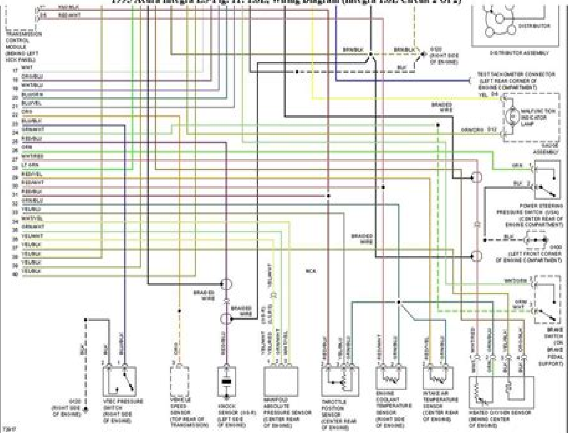
1995 Acura Integra LS- Fig. 11: LSL, Wiring Diagram (Integra LSL Circuit 2 Of 2)
