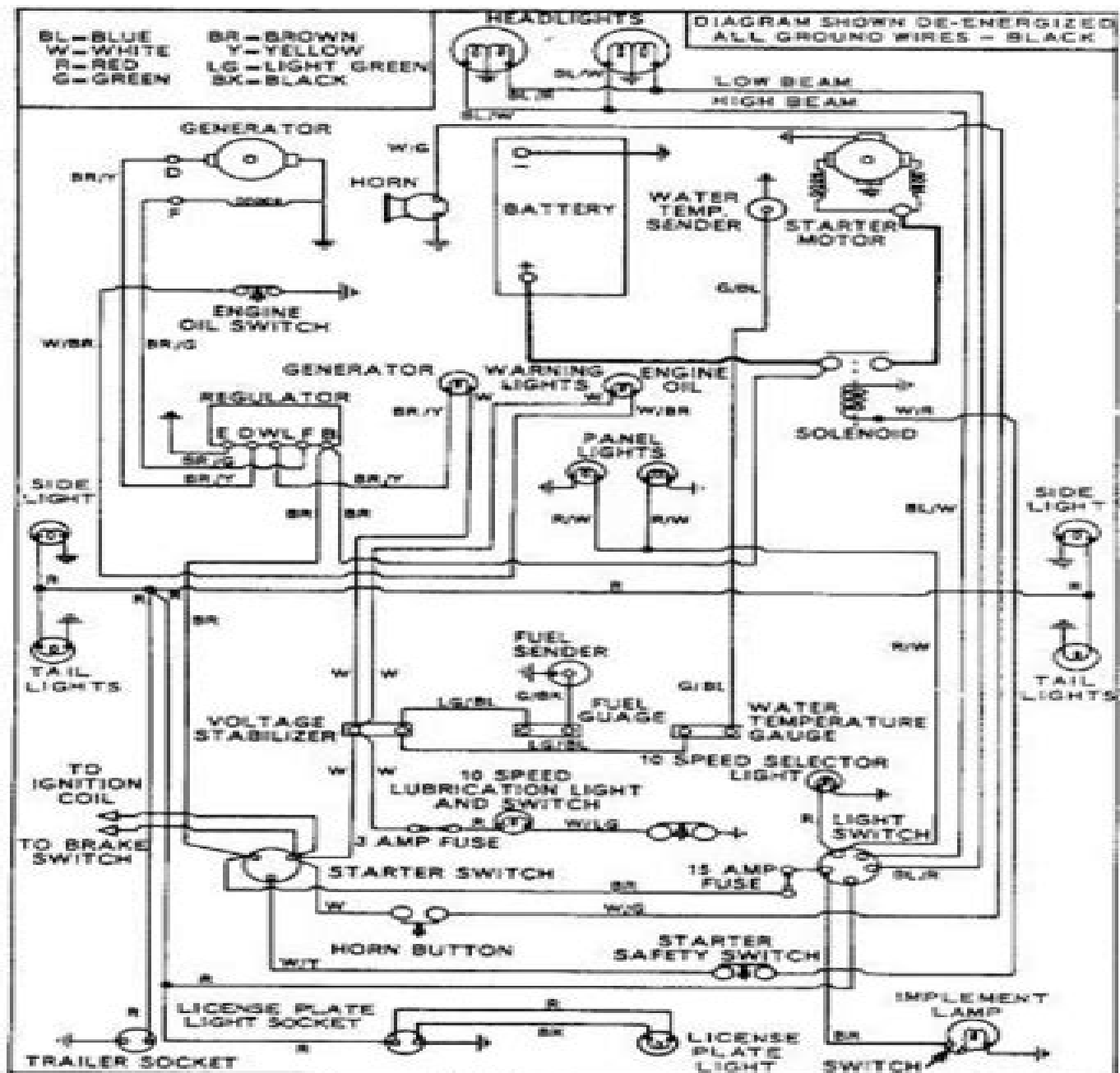
Fig. 161—Wiring diagram for all models with "A" or "B" prefix to tractor serial number. Refer to page 2 of this manual for serial number location. Refer to Fig. 160 for wiring diagram for models with "C" prefix.
