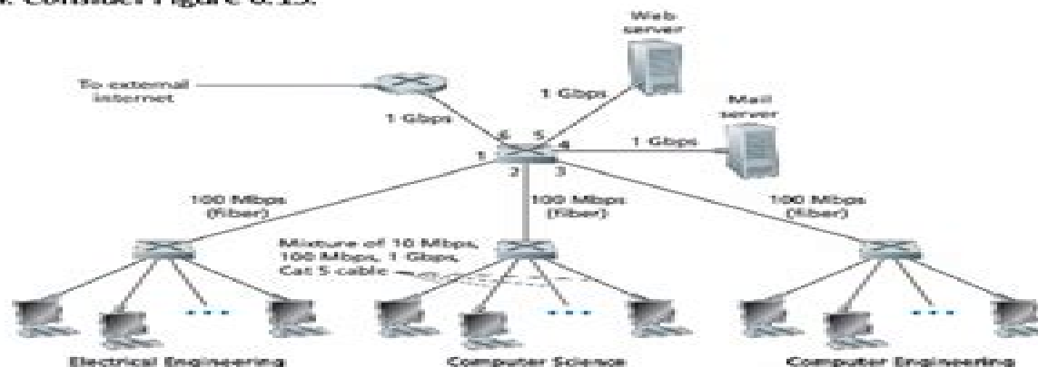
Figure 6.15 • An institutional network connected together by four switches
