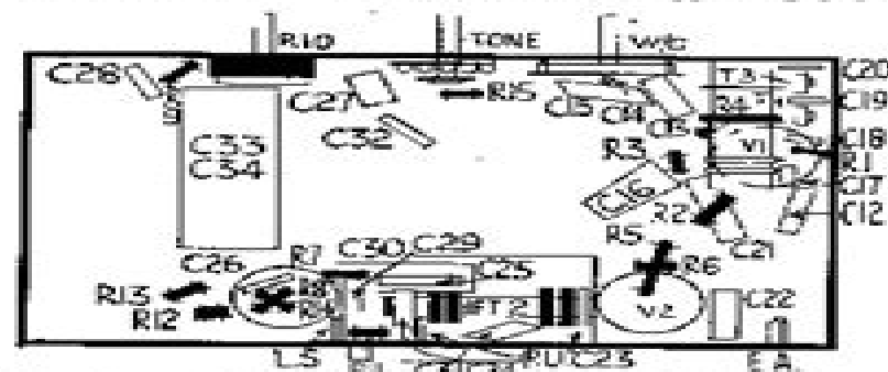
Layout diagrams of the MP chassis (prototype on right) identifying components. Condensers are in outline and resistors in solid black to aid reference.
