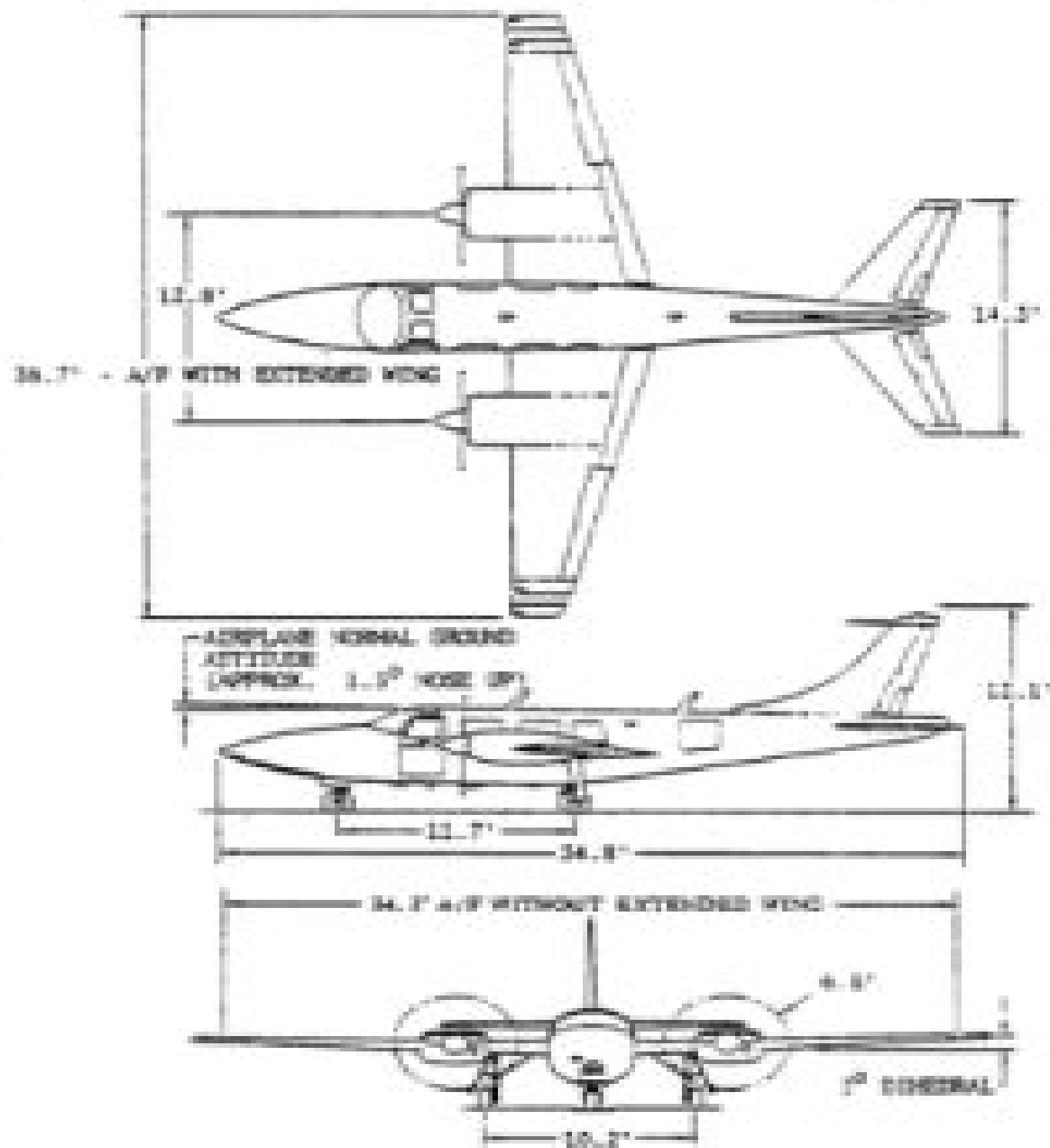
Figure 4-1. General Dimensions
