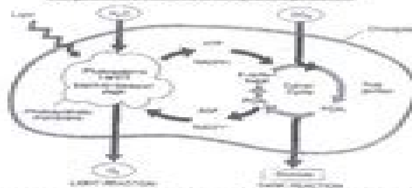
Diagram 1: Overview of photosynthesis
