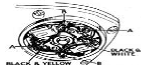
Breaker points (500 before H57083); sleeve nuts (A) and pillar bolts (B)
