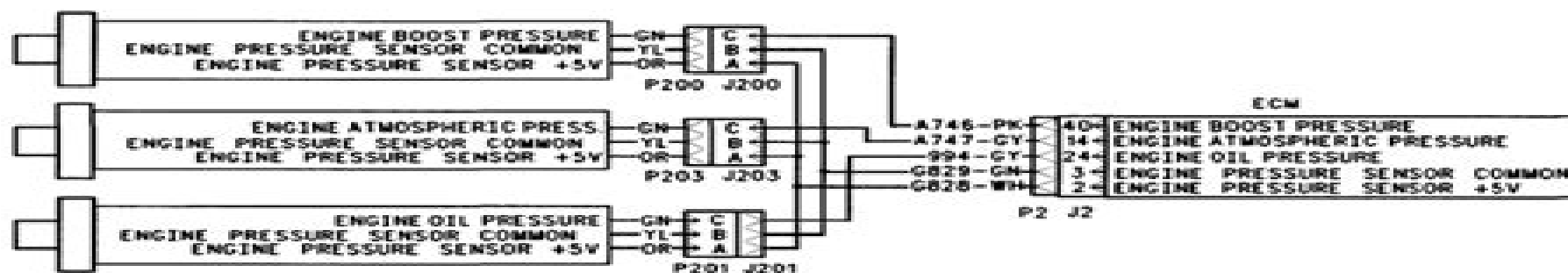
Illustration 103 Schematic for engine pressure sensors
