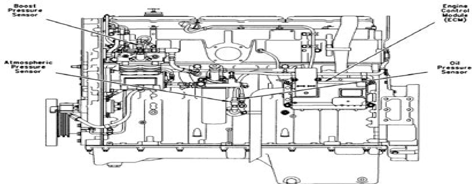
Illustration 102 C-15, C-16 and C-18 Pressure sensors
