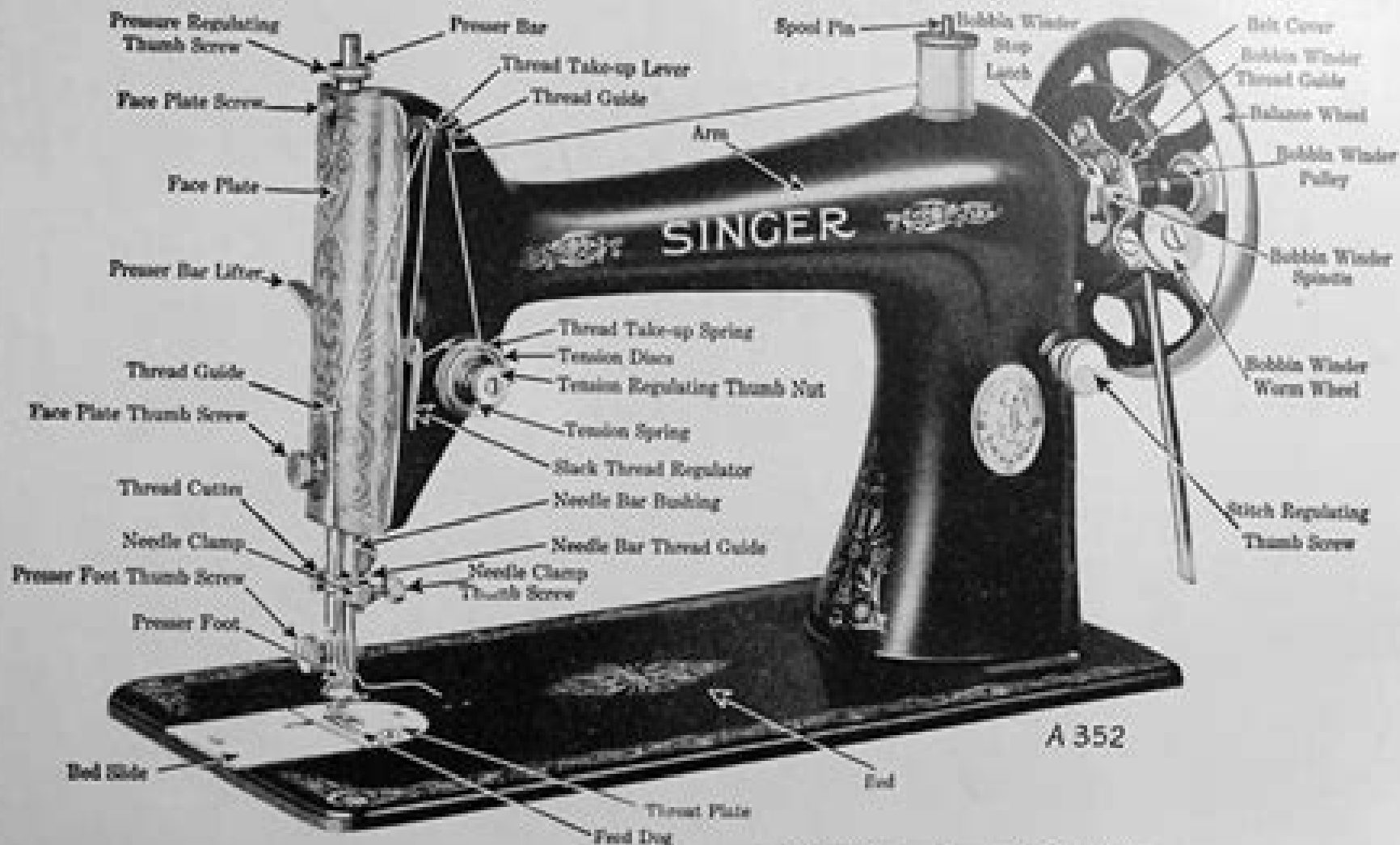
FIG. 43. NAMES OF PARTS OF THE HEAD—SINGER LOCK-STITCH MACHINES
