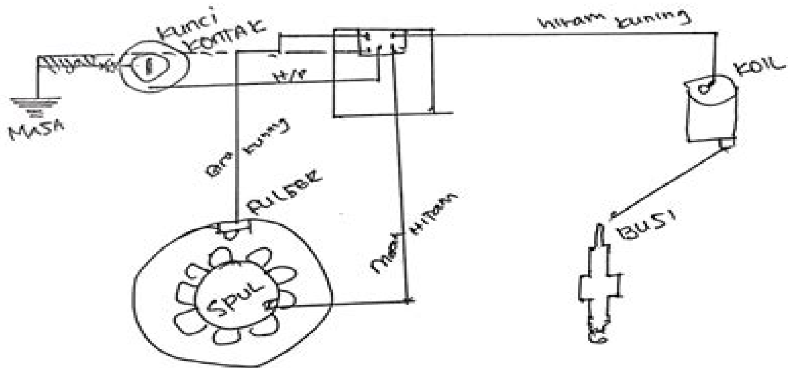
Gambar Diagram Rangkaian HONDA ERAND (m27anto.com)
